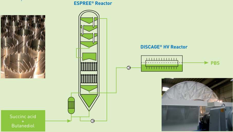
Figure 2: 2-stage PBS production process
